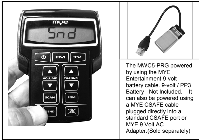
MWC5-98 Programmer
